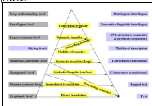
Figure 1: linguistic architectures of MT systems
